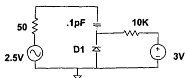
Fig. 4. Varactor circuit.
