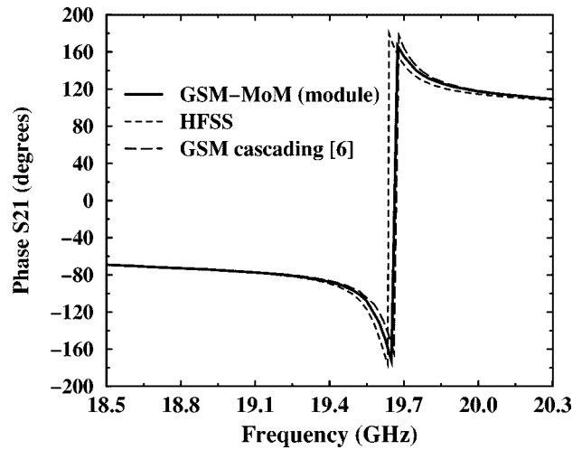
Fig. 5. Phase of the transmission coefficient S_{21} against frequency for a strip-to-slot transition module.
