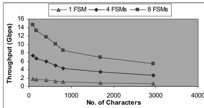
Fig. 7. Throughput for different character counts
