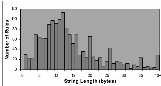
Fig. 5. Distribution of the string lengths in the Snort database
