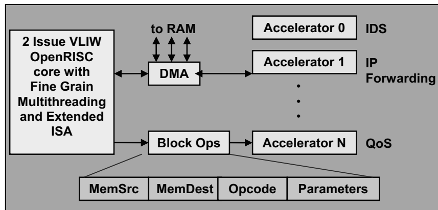
Fig. 3. Configurable network processor architecture
