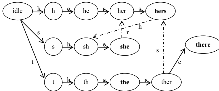
Fig. 2. Finite state machine diagram
