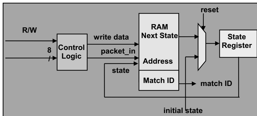
Fig. 4. String matching accelerator
