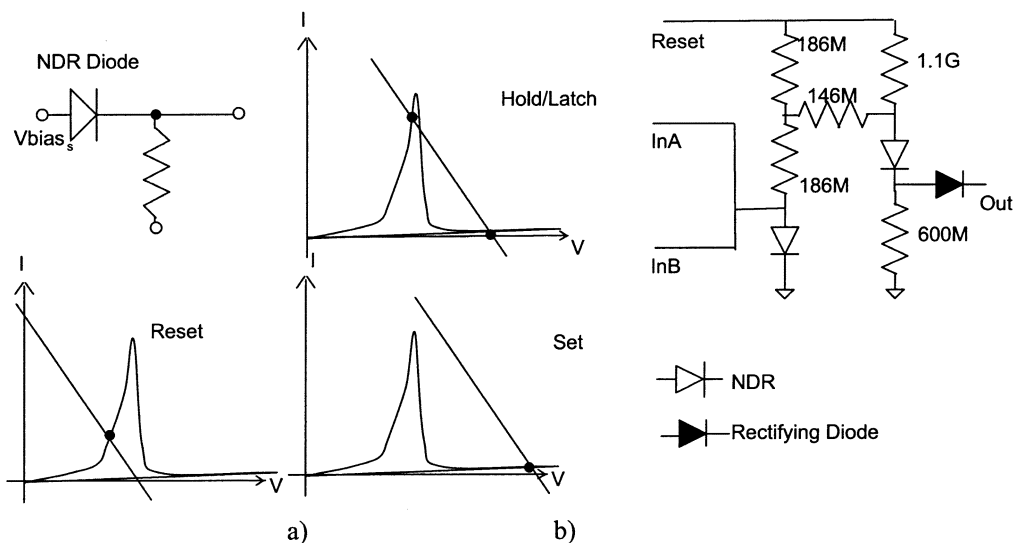
Fig. 8. (a) NDR latch, as used in memory circuits, and principle of operation. (b) NDR-based NAND gate.
