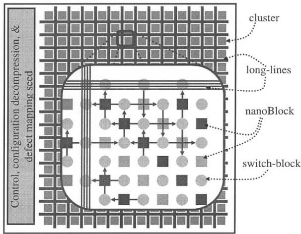
Fig. 17. The nanoFabric.
